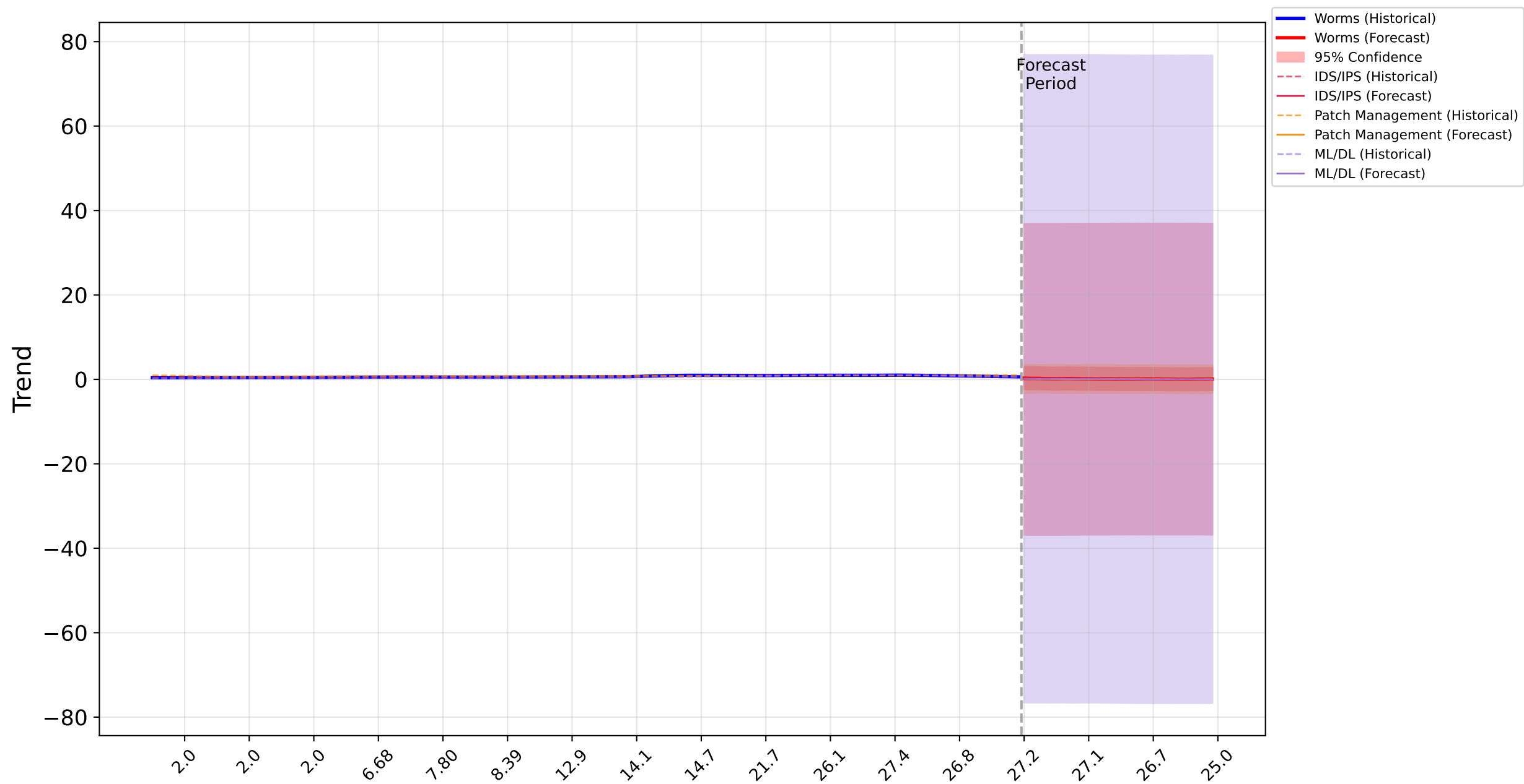
Worms Forecast Historical: 2.0 to 22.53454696505373 | Forecast: 2025-01 to 2027-12
